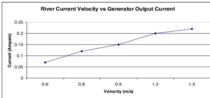
Figure 6. The correlation between river current velocity and generator output current.
